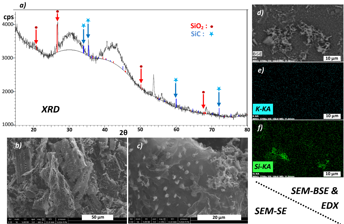
Figure 1: (a) XRD pattern and assignation of the SiO 2 and SiC peaks for KC-RS_3 sample, (b) and (c) SEM-SE pictures of KC-RS_3, (d) SEM-BSE picture of KC-RS_3, (e) and (f) EDX mapping of (d) for K and Si, respectively.
