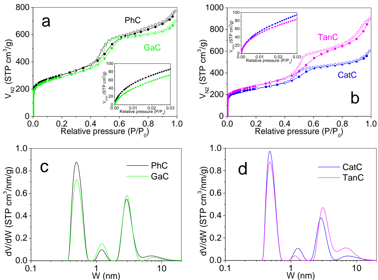
Figure 3. (a, b) Nitrogen adsorption-desorption isotherms and carbon dioxide adsorption isotherms (insets) of the ordered mesoporous carbons (OMCs); (c, d) corresponding pore size distributions.
