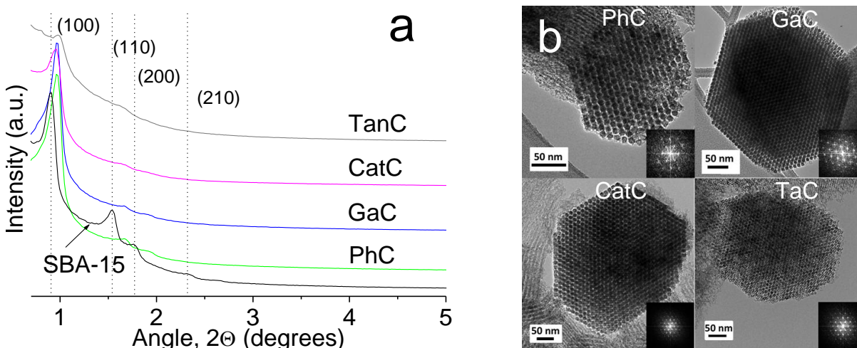
Figure 2. a) Small-angle X-Ray patterns of parent silica template and derived carbon materials; b) TEM and FFT (inset: Fast Fourier Transform) images of the carbon materials viewed along the cross-sectional direction of the rods.
