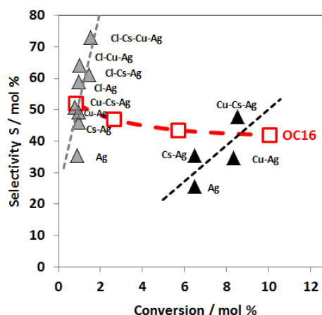
Figure 8. Comparison between OC16 (□ P=1\text{bar} , T = 448\text{-}523\text{ K} , C_2H_4/O_2=2 ) and materials from Jankowiak and Barteau [10] (▲ P=1.34\text{ bar} , T=540\text{ K} , C_2H_4/O_2=1 ); ▲ P=0.4\text{ bar} , T=479\text{-}540\text{ K} , C_2H_4/O_2=2 ). Ag stands for the reference material while Cs, Cu or/and Cl in the label stand for metal doping or chlorine treatment.
