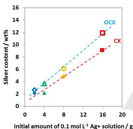
Figure 2. Silver content in the CX and OCX series of samples as a function of the initial amount of 0.1 M AgNO 3 in the HTC solution (◆ C2, ◆ OC2, ▲ C4, ▲ OC4, ● C8, ● OC8, ■ C16, ■ OC16).
