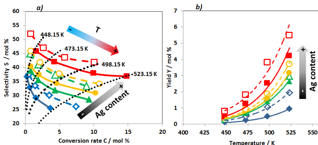
Figure 5. (a) Selectivity of the catalyst versus conversion rate at 4 different temperatures, and (b) reaction yield versus temperature for the two series of samples CX and OCX. The lines are just guides for the eye (♦ C2, ♦ OC2, ▲ C4, ▲ OC4, ● C8, ● OC8, ■ C16, ■ OC16).
