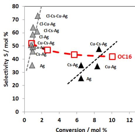
Figure 8. Comparison between OC16 (□) ( P=1\text{bar} , T = 448\text{-}523\text{ K} , C_2H_4/O_2=2 ) and materials from Jankowiak and Barteau [10] (▲) ( P=1.34\text{ bar} , T=540\text{ K} , C_2H_4/O_2=1 ); ▲ ( P=0.4\text{ bar} , T=479\text{-}540\text{ K} , C_2H_4/O_2=2 ). Ag stands for the reference material while Cs, Cu or/and Cl in the label stand for metal doping or chlorine treatment.
