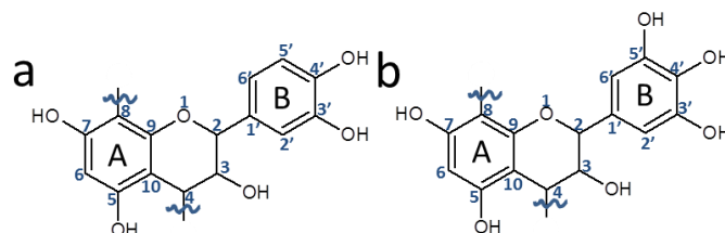
Scheme 1. Chemical structure of the flavonoid unit of a pine condensed tannin: (a) procyanidin; (b) prodelphinidin.
