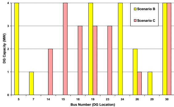
Fig. 2: Optimum location and sizing of DG (case I).
