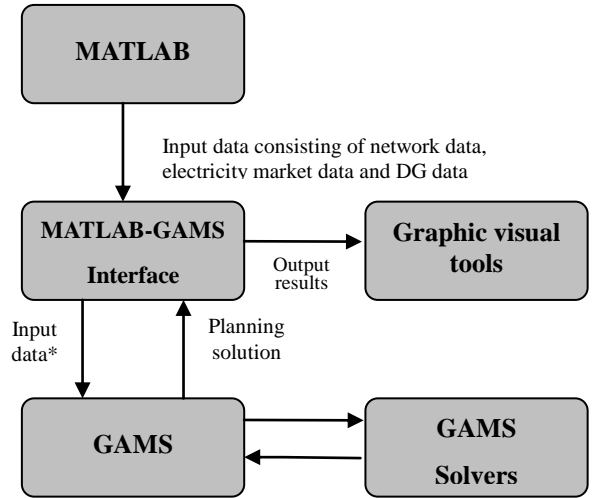
Fig. 1: MATLAB-GAMS interface
