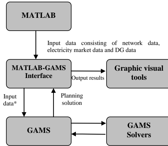
Fig. 2: MATLAB-GAMS interface.
