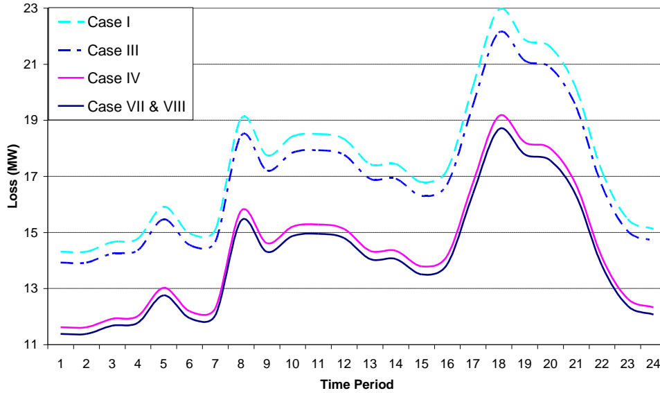
Fig. 17: Total system losses versus time period in cases I, III, IV, VII&VII
