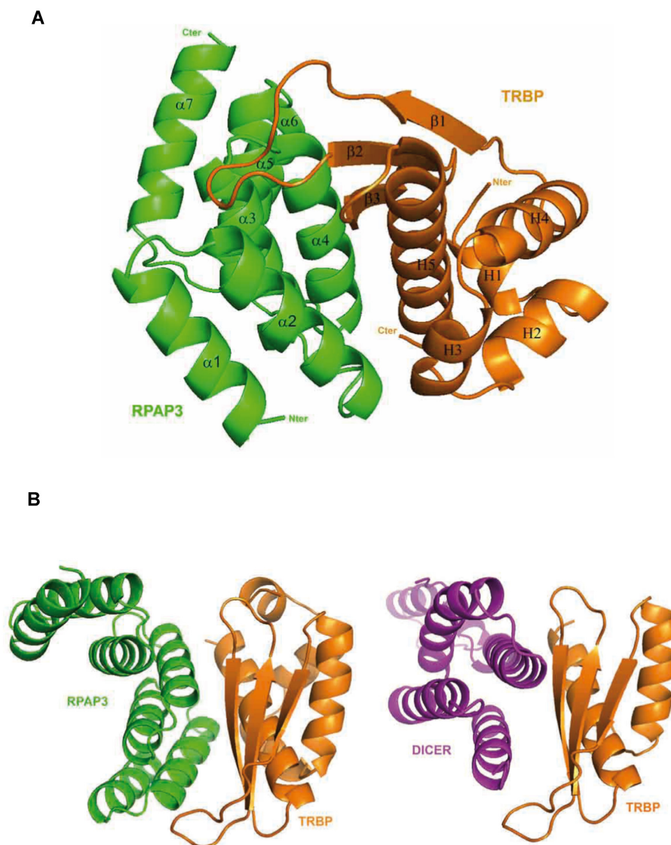
Figure 4. Crystal structures of the TRBP:RPAP3 complex. (A) Ribbon representation of the X-ray crystallographic structure of the TPR1 domain of RPAP3 and the dsRBD3 of TRBP at 1.49 Å resolution. RPAP3 (residues 133–249) and TRBP (residues 263–365) are drawn in green and orange, respectively. (B) Ribbon representations of our crystal structure (left) and the one published by Wilson et al. (10) (right) confirm that TRBP shares the same binding interface for its interaction with either Dicer or RPAP3.
