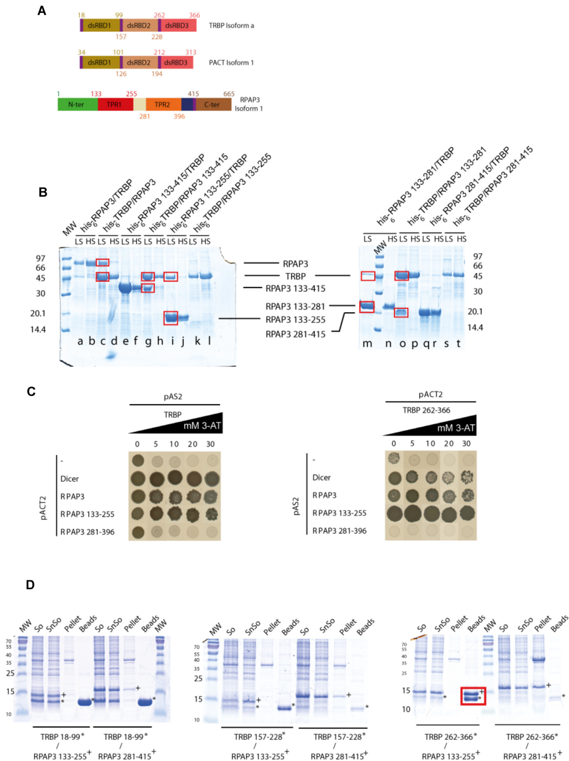
Figure 2. Identification of the protein subdomains involved in the interaction. (A) Representation of the subdomains of TRBP and RPAP3 as predicted with the software IUPRED and PSIPRED (61,62). Numbers correspond to the amino acid residues located at each domain extremities. (B) Co-expression and co-purification experiments in E. coli performed with RPAP3, TRBP and their subdomains. For each protein pair, the first protein name on top of the gel always indicates the His 6 -tagged protein. The beads were directly resuspended in 2x Laemmli buffer and fractionated on 15% SDS-PAGE. Positive interactions are highlighted with red squares. (C) Two-hybrid screens performed in the yeast S. cerevisiae on TRBP, RPAP3 and their subdomains. The TRBP:Dicer interaction was used as a positive control. pAS2 and pACT2 plasmids respectively enable expression of a protein fusion with the DNA binding domain or activation domain of transcription factor Gal4. Strengths of the interactions were tested using increasing amounts of 3-amino-triazol (3-AT) from 0 to 30 mM. (D) Purification steps of co-expression experiments in E. coli performed with RPAP3 (*) and TRBP (+) subdomains and analyzed by SDS-PAGE. The TRBP and RPAP3 domains used are indicated below the gel lanes. The TRBP subdomains carried the His 6 -tag. 'So', 'SnSo', 'Beads', 'MW' and 'Pellet' design respectively the culture sonicate, supernatant sonicate, Talon beads, Molecular Weight marker and sonicate pellet. The positive interaction (dsRBD3 of TRBP and TPR1 of RPAP3) is highlighted with a red square. None of the TRBP domains interacted with the TPR2 of RPAP3.
