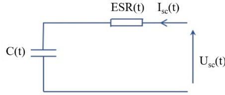
Figure 3. Thevenin electrical model of the SC.
