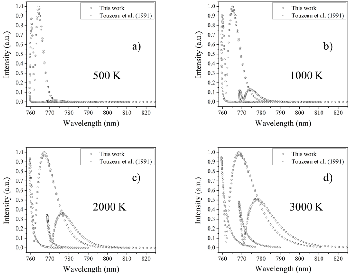
Figure 14: Theoretical intensity of the O_2(b^1\Sigma_g^+, v'=0) \rightarrow O_2(^3\Sigma_g^-, v''=0) and O_2(b^1\Sigma_g^+, v'=1) \rightarrow O_2(^3\Sigma_g^-, v''=1) transitions of the O_2 atmospheric band. Comparison between the present set of data and the one given by Touzeau et al. (1991).
