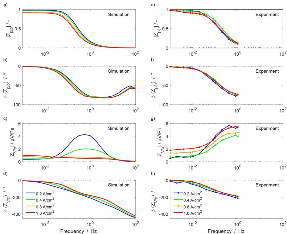
Figure 5. Bode plot of simulated (solid lines) and experimental (solid lines with circles) pressure impedance spectra at different current densities. (a), (b), (e), (f) Transfer function Z_{pp} , ratio between cathode inlet and outlet pressure oscillation. (c), (d), (g), (h) Transfer function Z_{V/p} , electrochemical pressure impedance. The data at 0.4 \text{ A/cm}^2 have been published before. 18
