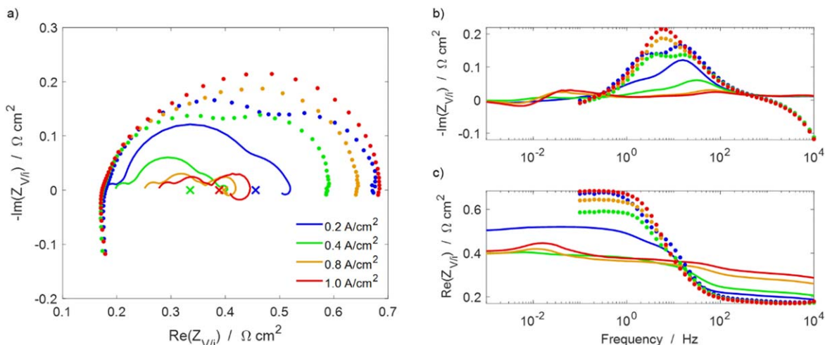
Figure 3. Experimental (solid circles) and simulated (solid lines) electrochemical impedance spectra Z_{VII} in (a) Nyquist and (b), (c) Bode representation for different current densities between 0.2 and 1.0 \text{A cm}^{-2} . The experimental DC resistance (gradient of the polarization curve) is plotted on the real axis of the Nyquist plot (crosses). The operating conditions are the same as for the polarization experiments shown in Fig. 2.
