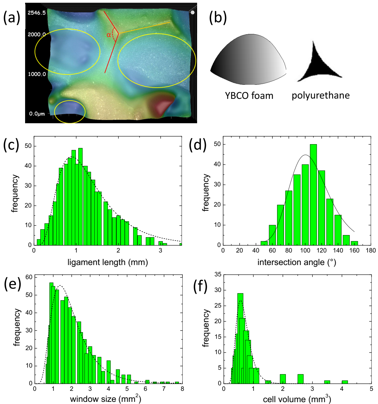
Figure 7. (a) Definitions of the ligament length (orange arrow), the intersection angle \alpha (red arrow) and the window size (yellow ellipses). (b) presents the typical cross section found by profile analysis for the YBCO foam (left) compared to a sketch of the cross section following Jang et al. [22]. (c–f) Statistical distribution analysis of the ligament (strut) lengths, the window size, the intersection angles and the cell size. The black dashed lines indicate log-normal fits to the data, and a normal fit in (d).
