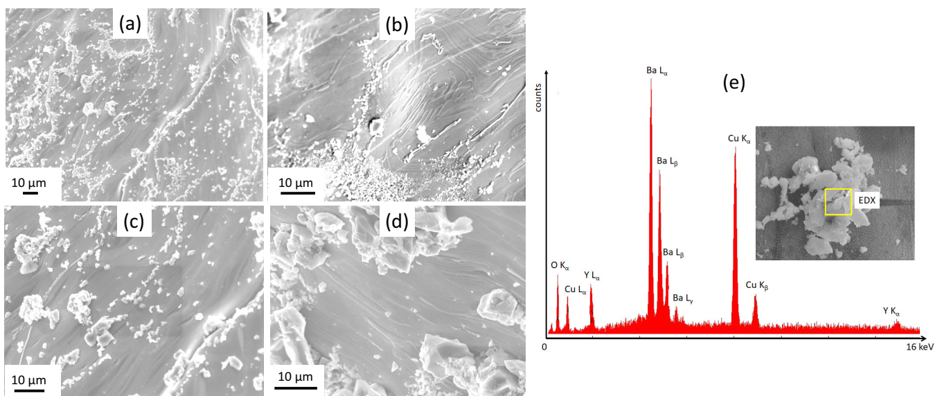
Figure 3. (a–d) SEM images (various magnifications ranging between 650\times and 2200\times ) showing details of the internal surfaces of the foam struts and vertices. The particles seen on the strut surfaces are \text{Ba}_3\text{Cu}_5\text{O}_y particles as determined by EDX analysis (e). These structures and particles are caused by the capillary flow of the liquid phase during IG-processing, which is not seen in conventional bulk samples.
