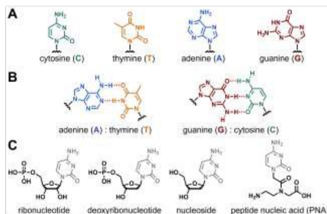
Fig. 1 (A) Chemical structures of nucleobases and (B) the two canonical Watson-Crick base pairing. (C) Chemical structures of nucleobase-containing moieties.
