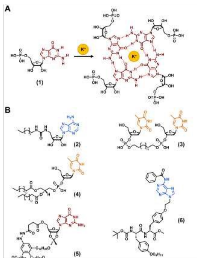
Fig. 2 (A) G-quartet formation from the guanosine-5'-monophosphate ( 1 ). (B) Chemical structures of nucleobase-containing compounds able to form hydrogels (( 2 ) 110 , ( 3 ) 111 and ( 4 ) 112 ) or organogels (( 5 ) 113 and ( 6 ) 68 ).
