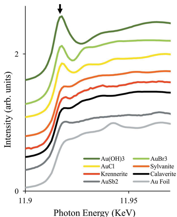
Figure 7 Au L_{III} -edge and Te K -edge XANES spectra for calaverite, krennerite, sylvanite and reference Au materials. The arrow indicates the white line at the absorption edges.
