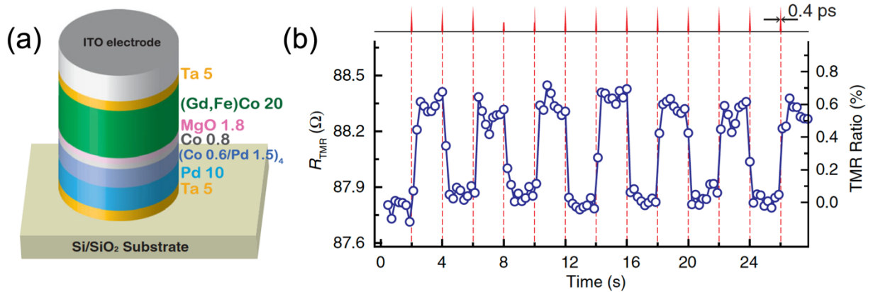
Figure 3: (a) Schematic of the MTJ stack employing Gd 26 (Fe 90 Co 10 ) 74 as the free layer and Co/Pd ML as the reference layer, (b) HI-AOS of the 12 nm MTJ cell measured via TMR electrical read-out as reproduced with the permission from Chen et al. , 57 copyright 2017 AIP Publishing.
