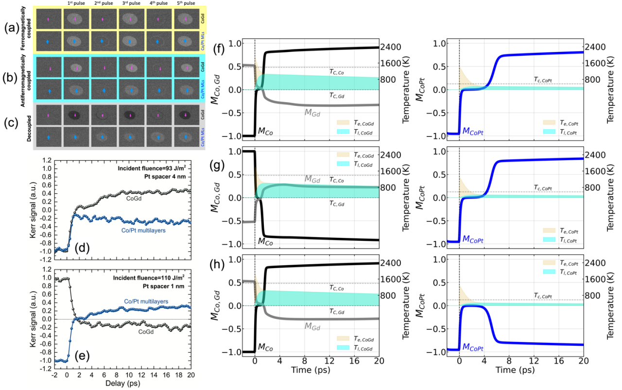
Figure 2: (a-c) Depth sensitive single-shot MOKE micrographs of the (a) ferromagnetically, (b) anti-ferromagnetically and (c) decoupled FM-FEM stack. (d-e) Depth-sensitive time resolved magnetization dynamics of Co/Pt and CoGd for decoupled (d) and ferromagnetically coupled (e) stacks. (f-h) The simulated magnetization dynamics of Co, Gd, and Co/Pt sublattice simulated for ferromagnetically, anti-ferromagnetically and decoupled FM-FEM stack and the time-evolution of corresponding electron and lattice temperature using the extended M3TM model and the corresponding evolution of electron and phonon temperatures are shown by light yellow and cyan filled regions, respectively, and the Curie temperatures of Co and Co/Pt are shown by the dotted lines as taken from 60 . Reprinted with permission from the authors.
