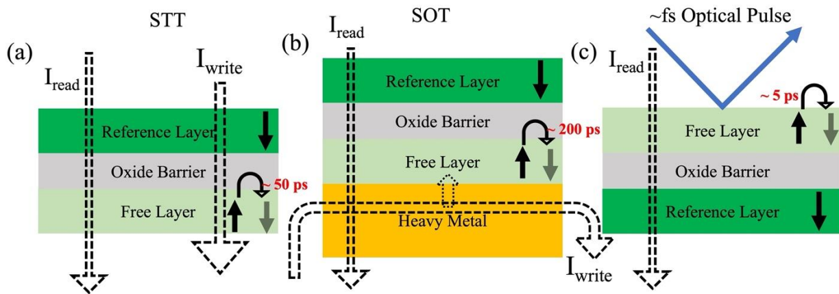
Figure 1: The schematic of a basic MTJ cell employing (a) STT, (b) SOT mechanism, and (c) femtosecond pulse excitation
