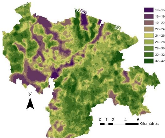
Figure 4. Amplitude thermique diurne ( T^{\circ}C )
