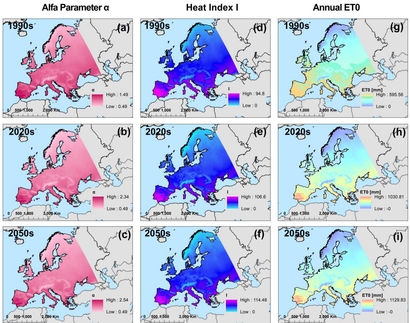
Figure 3. Spatial distribution of Alfa parameter ( \alpha ), heat index ( I ), and annual potential evapotranspiration (ET0) in Europe. (a) Alfa parameter \alpha in 1990s. (b) Alfa parameter \alpha in 2020s. (c) Alfa parameter \alpha in 2050s. (d) Heat index I in 1990s. (e) Heat index I in 2020s. (f) Heat index I in 2050s. (g) Annual ET0 in 1990s. (h) Annual ET0 in 2020s. (i) Annual ET0 in 2050s.
