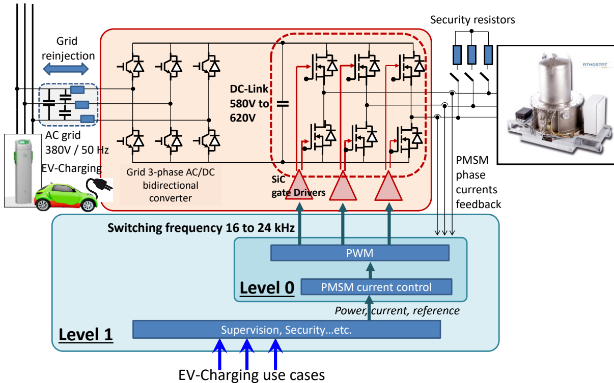
Figure 1. General overview of the FESS (Flywheel Energy Storage System) used for EV-charging
