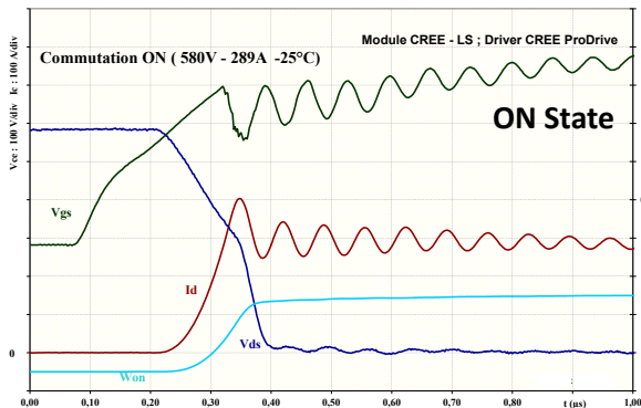
Figure 5.a) SiC MOSFET switching ON state
