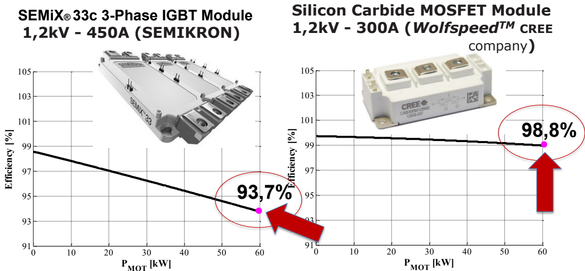
Figure 4. Comparison of the efficiencies for Silicon and Silicon carbide (SiC) semiconductor modules according to motor system’s power (kW)
