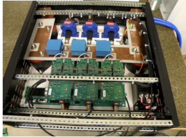
Figure 8. DC-AC Inverter prototype on heatsink (with DC busbar, current LEM© sensors, capacitor's snubber and interface driver cards for CREE ProDrive®). The DC-AC inverter is water cooled
