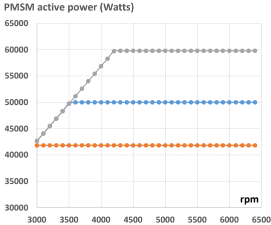
Figure 2. PMSM power profile with current limitation
