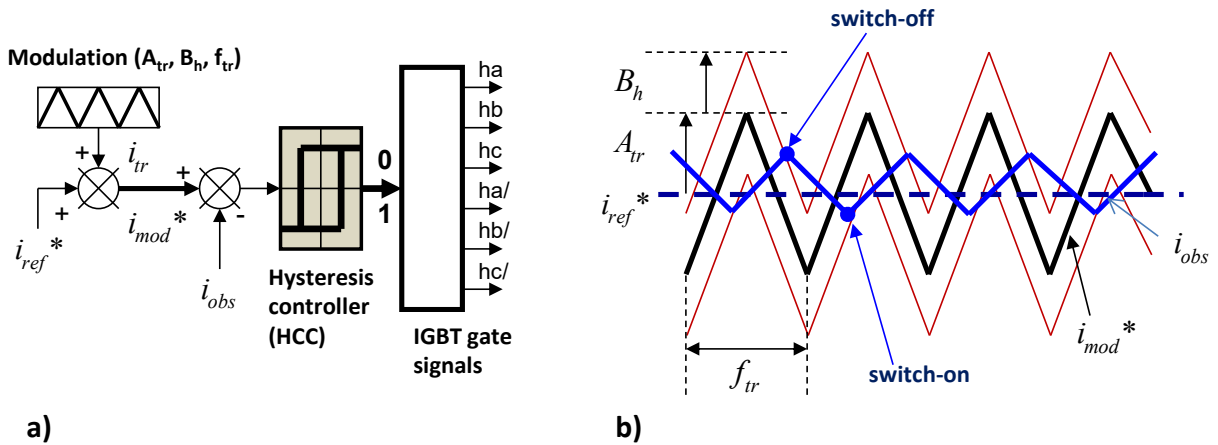
Figure 10. Modulated hysteresis method
