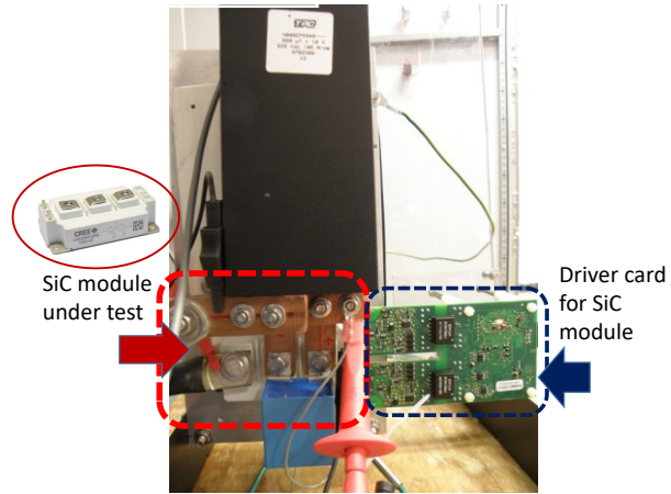
Figure 3. Fig. 3: Experimental set-up for HF switching test of the SiC 1200V/300A Half-Bridge with driver card
