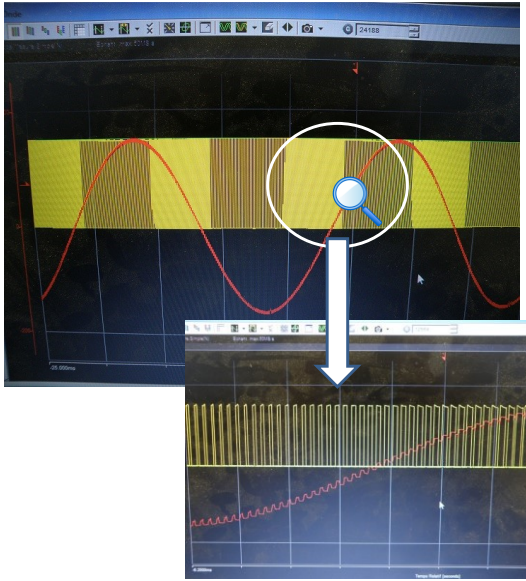
Figure 7. Focus on 20kHz PWM gate signal and AC phase current (view on digital scope recorder)
