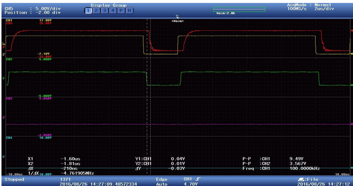
Figure 6.b) Driver card Prodrive® gate output Switching results up to 100 kHz
