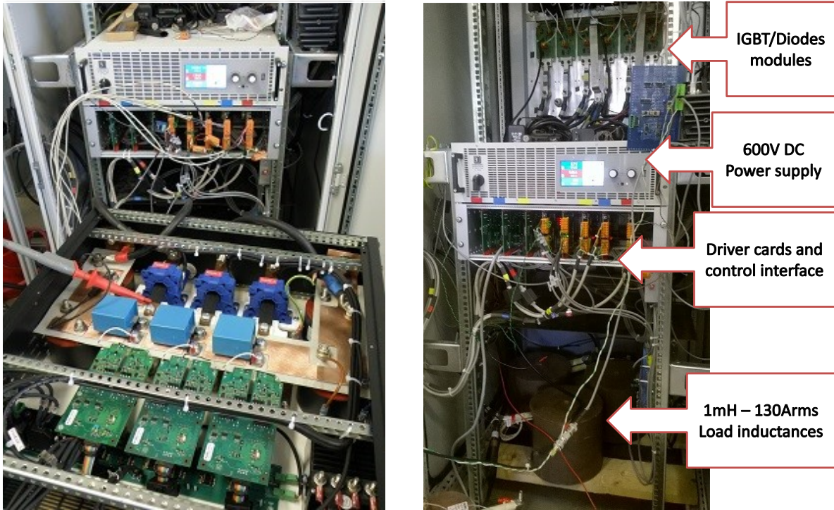
a) SiC converter under test connected to the test bench
