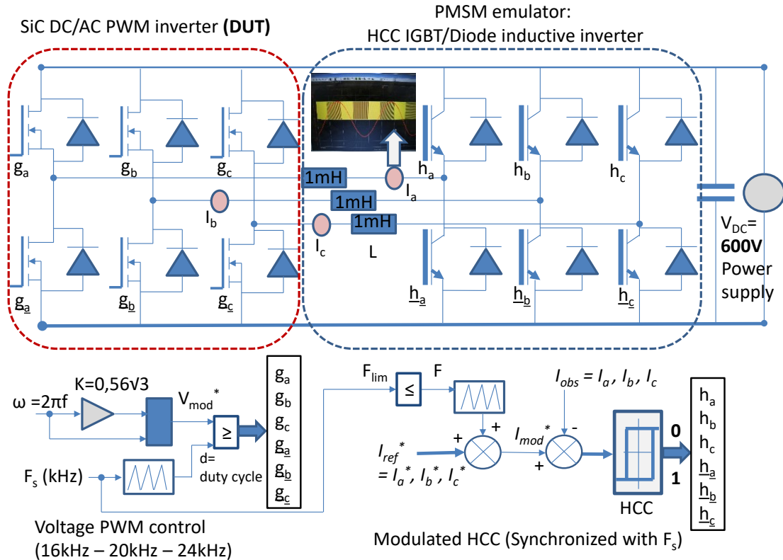
Figure 9. Electrical topology for DC-AC SiC inverter connected to the double-converter architecture
