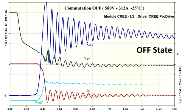
Figure 5.b) SiC MOSFET switching OFF state
