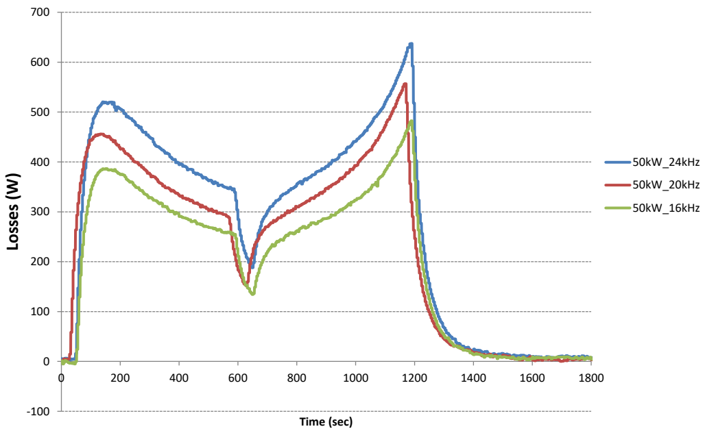
Figure 13. Experimental thermal losses for 50kW speed up and down profile
