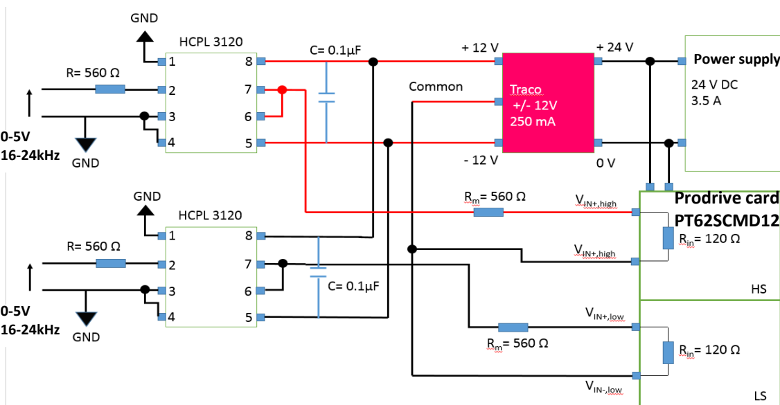
Figure 6.a) Driver interface synopsis with HCPL-3120 optocoupler for one SiC inverter leg
