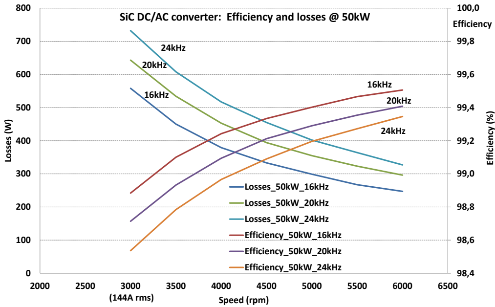
Figure 12. Experimental thermal losses for 50kW test Thermal losses (W) for speed cycle
