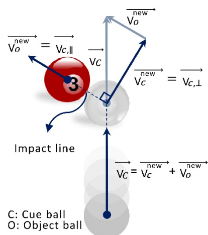
Figure 1. Velocity components of billiards balls after a collision that is inspiring for BOA [13].
