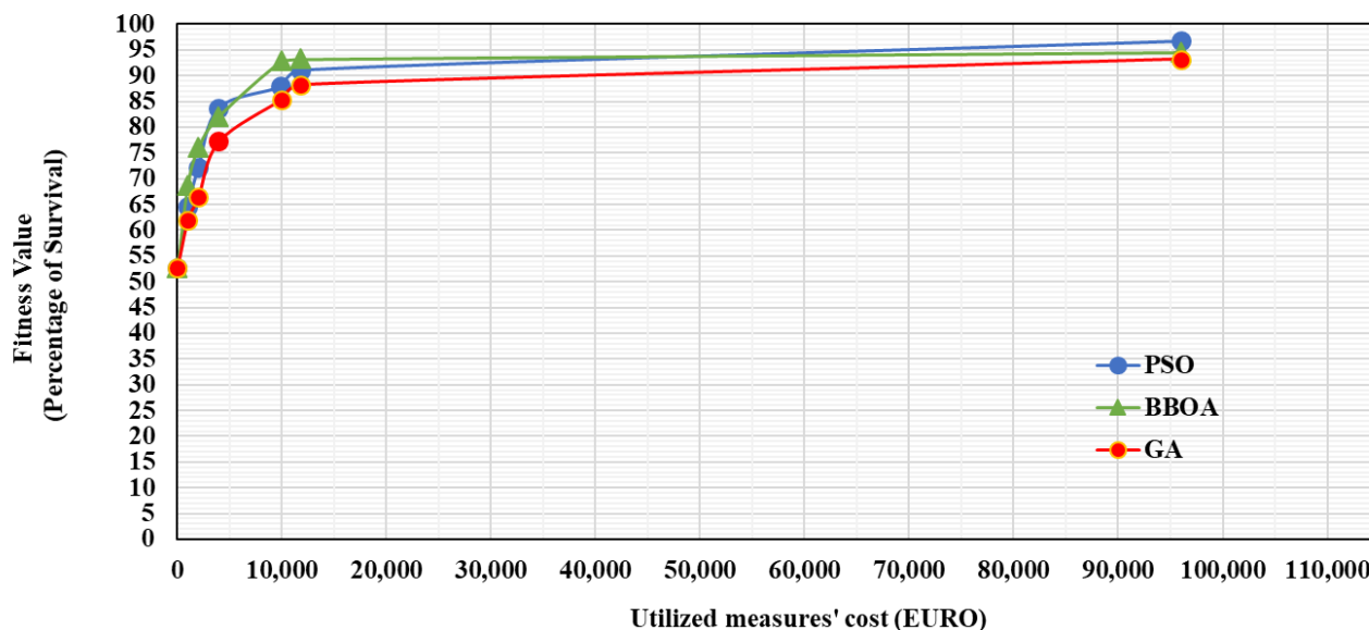
Figure 21. Comparison of optimisation algorithms results for the hospital building.
