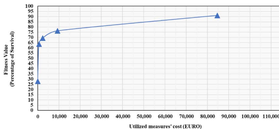
Figure 22. Optimisation algorithms results for the residential building.
