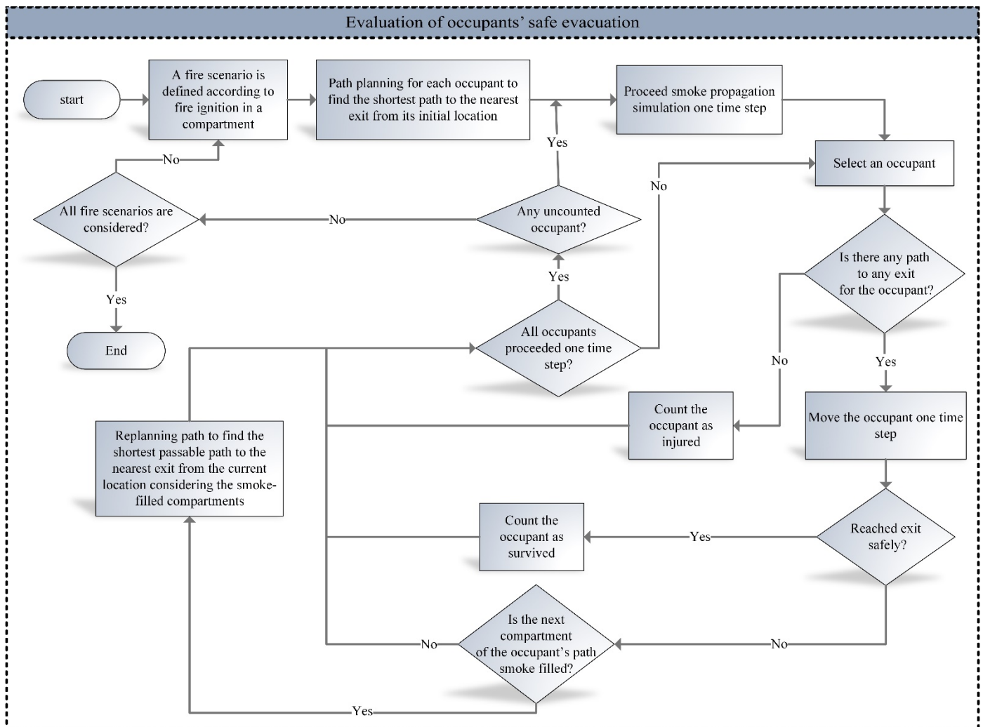
Figure 9. Evaluation of occupants' safe evacuation.
