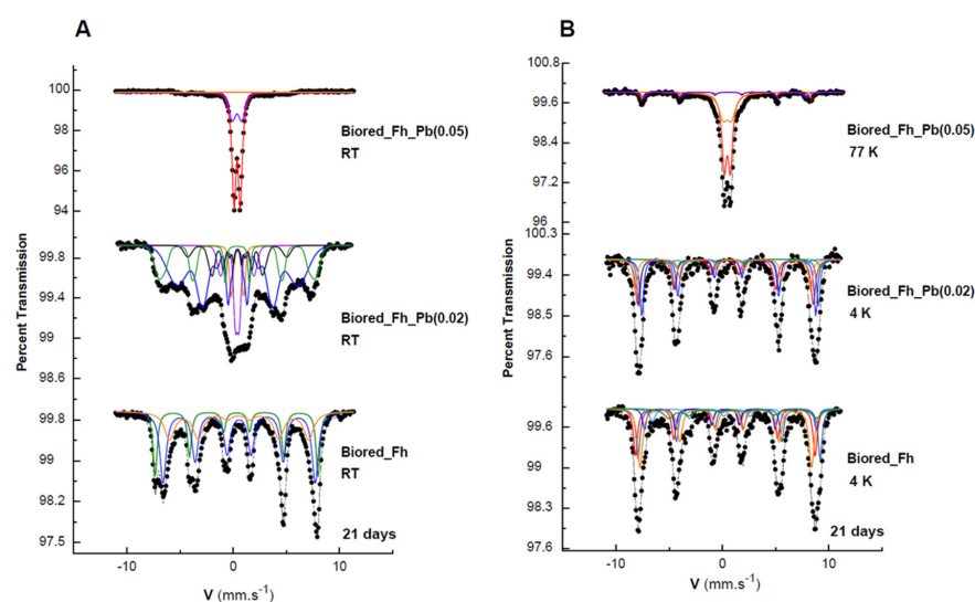
Figure 5. Mössbauer spectra of the secondary products obtained in the Fh, Fh_Pb(0.02), and Fh_Pb(0.05) systems at: (A) room temperature (RT), and (B) 77 or 4 K after the RP2 with Shewanella oneidensis MR-1. Hyperfine parameters corresponding to these spectra are presented in Table 2.
