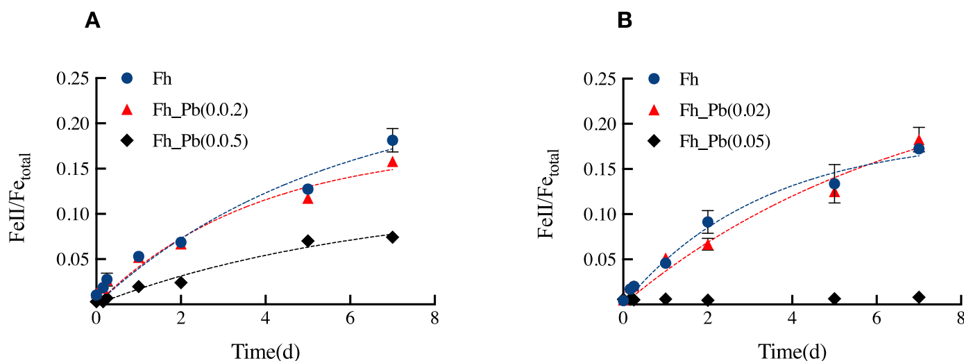
Figure 1. Concentrations of Fe(II) ions formed in the Fh, Fh_Pb(0.02), and Fh_Pb(0.05) systems during: (A) the RP1, and (B) the RP2 with Shewanella oneidensis MR-1. Error bars indicate the standard deviations of triplicate microbial-reduction assays.
