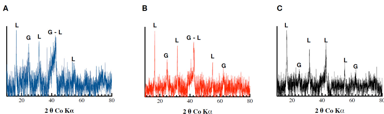
Figure 2. Diffractograms obtained following Co-XRD measurements of the (A) Fh, (B) Fh_Pb(0.02), and (C) Fh_Pb(0.05) systems after the RP1 with Shewanella oneidensis MR-1.
