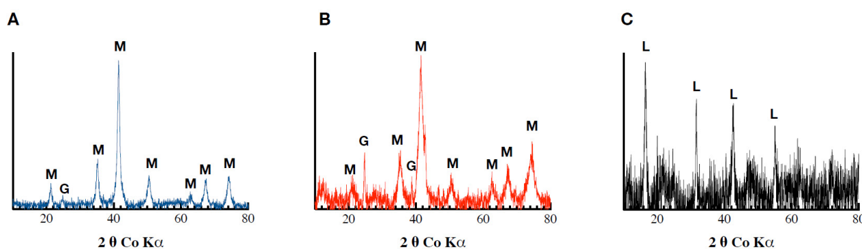
Figure 4. Diffractograms obtained following Co-XRD measurements of the (A) Fh, (B) Fh_Pb(0.02), and (C) Fh_Pb(0.05) systems after the RP2 with Shewanella oneidensis MR-1.
