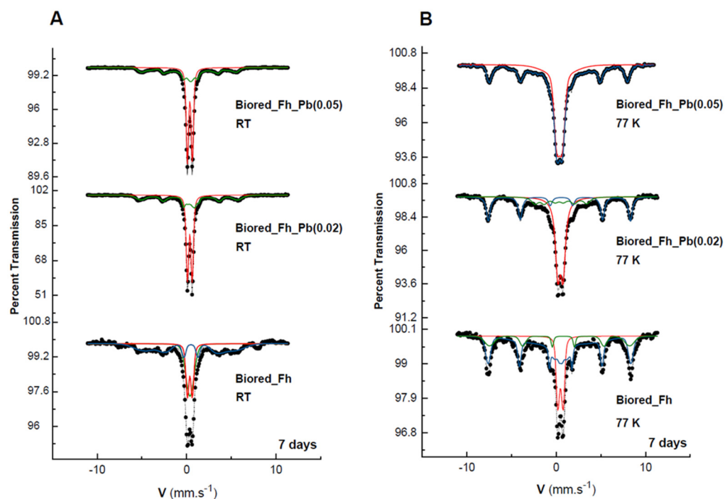
Figure 3. Mössbauer spectra of the secondary products obtained in the Fh, Fh_Pb(0.02), and Fh_Pb(0.05) systems at: (A) room temperature (RT), and (B) 77 K after the RP1 with Shewanella oneidensis MR-1. Hyperfine parameters that correspond to these spectra are presented in Table 1.
