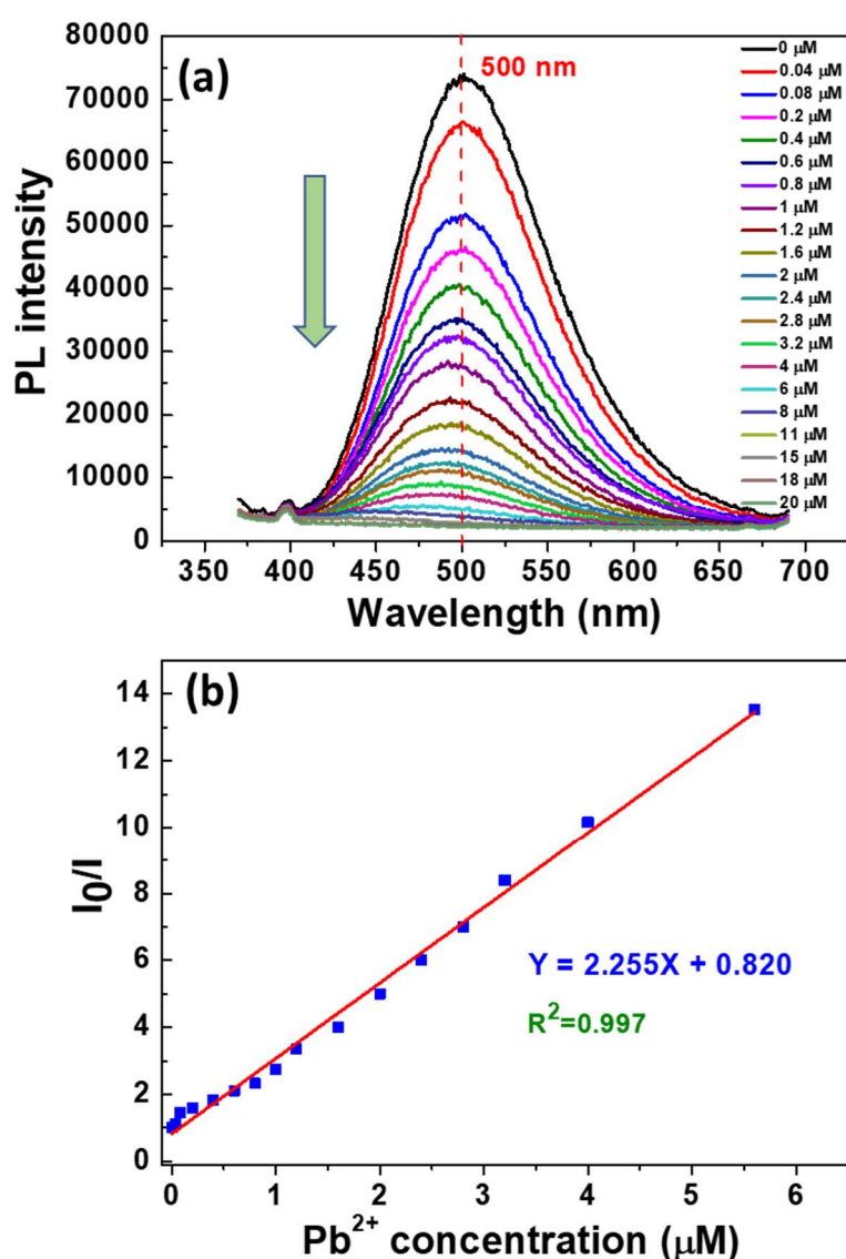
Fig. 4. (a) PL emission spectra of ZnSeS/Cu:ZnS/ZnS QDs dispersed in water upon addition of various concentrations of Pb 2+ , (b) the linear correlation of I_0/I vs the concentration of Pb 2+ in the range 0.04-6 \mu\text{M} .
