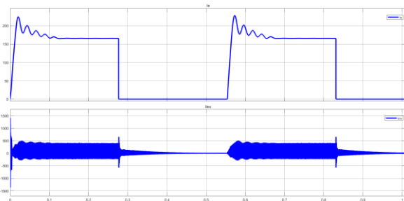
Figure 4: DC current before and after the LCLC filter
