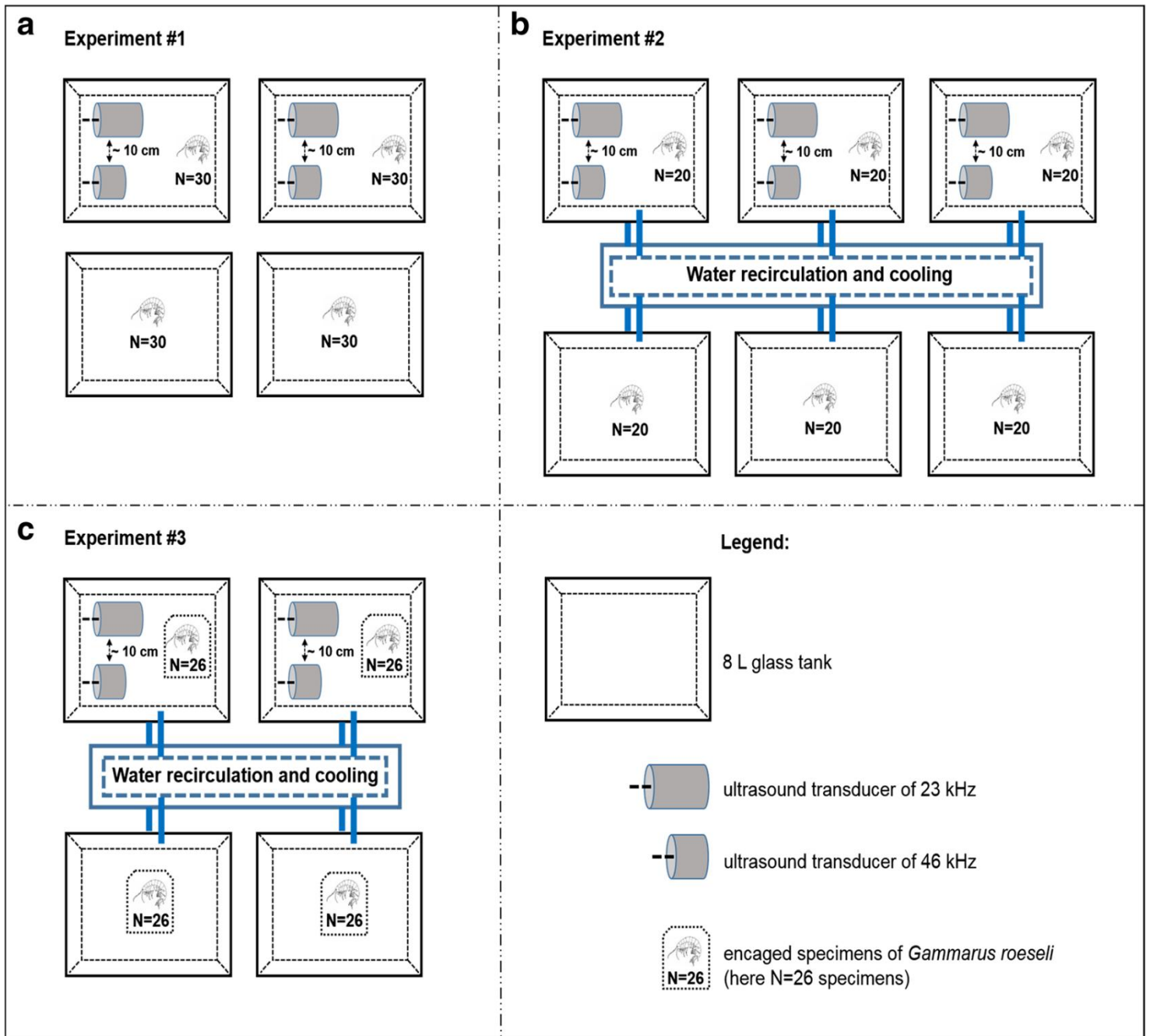
Figure 2. Ultrasonic experimental setup.
