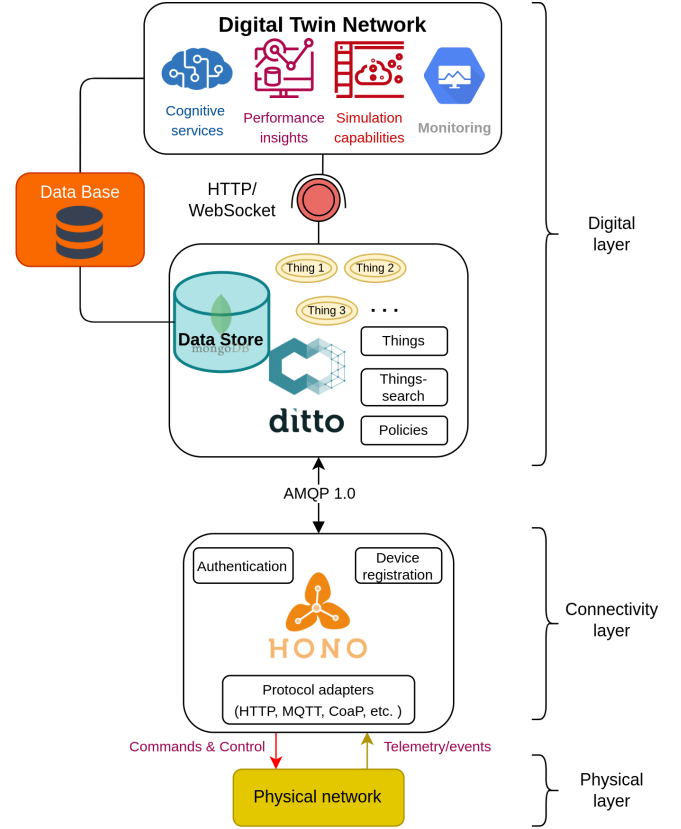
Fig. 1. Digital Twin Network using Eclipse Ditto + Hono.
