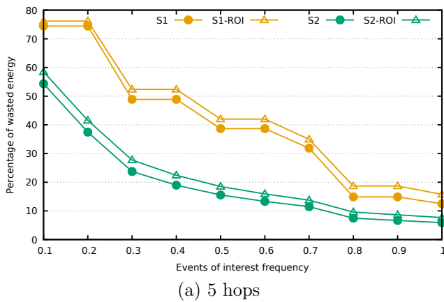
Fig. 8. Percentage of wasted energy
