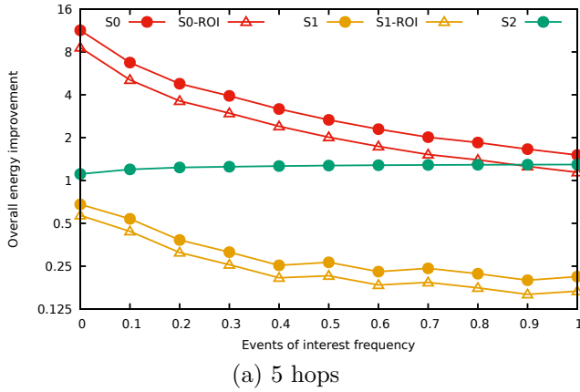
Fig. 7. Improvement of overall consumed energy
