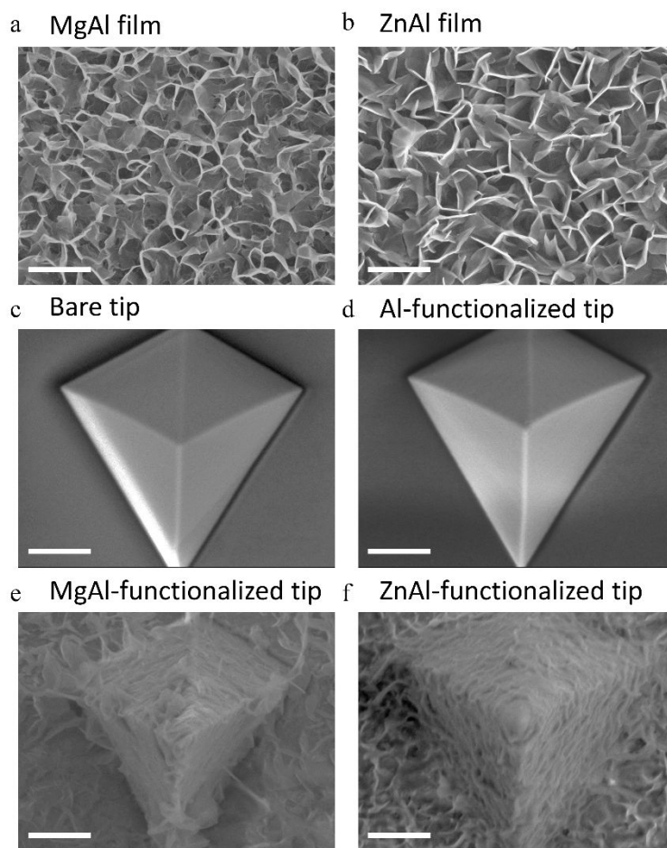
Figure 4. SEM images of LDH films on silicon wafers and AFM tips (scale bar = 1 \mu m). (a) MgAl LDH film grown on silicon wafer. (b) ZnAl LDH film grown on silicon wafer. (c) Bare silicon nitride AFM tip. (d) Al-functionalized silicon nitride AFM tip. (e) MgAl LDH-functionalized silicon nitride AFM tip. (f) ZnAl LDH-functionalized silicon nitride AFM tip.
