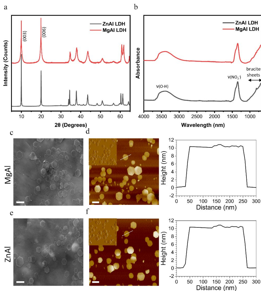
Figure 1. NPs characterization. (a) XRD patterns of MgAl and ZnAl NPs. (b) FT-IR spectra of MgAl and ZnAl NPs. (c,e) SEM images of MgAl (c) and ZnAl (e) NPs (scale bar = 200 nm). (d,f) AFM height images of MgAl (d) and ZnAl (f) NPs (scale bar = 200nm, insets are deflection images showing the NPs surface ultra-structure) together with height profiles of single particles. Dashed lines marked on the height images represent the sections used to determine the height profiles.
