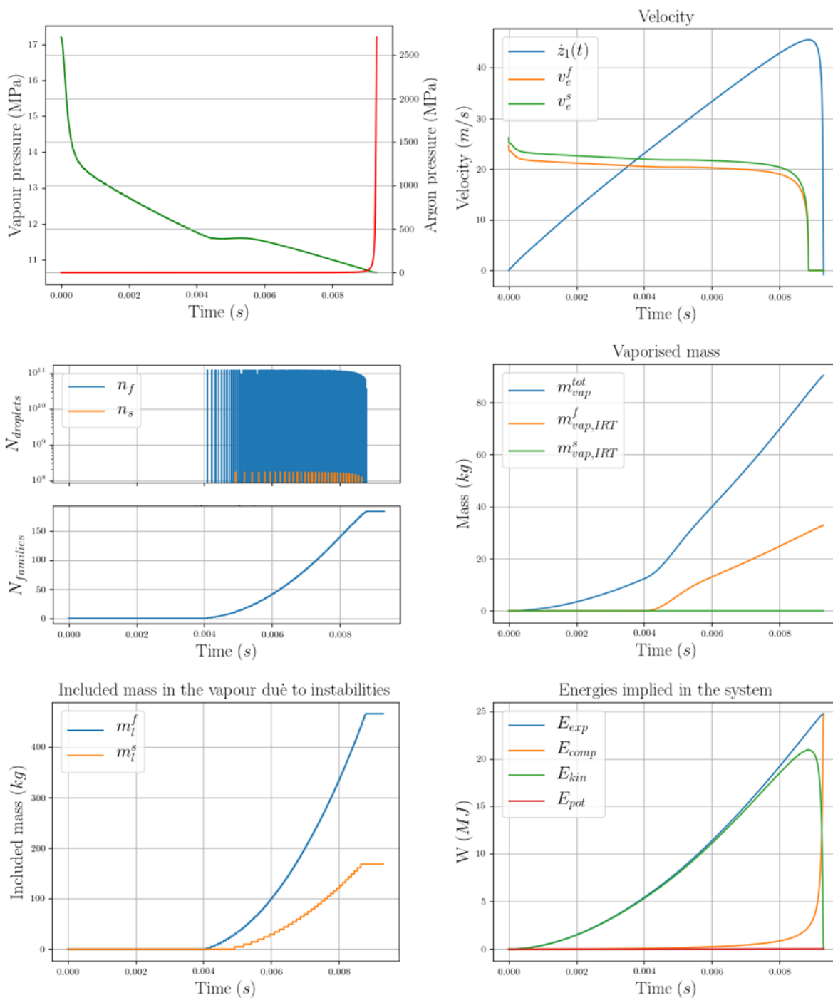
Figure 5. Relevant values during the MOREINa's transient with instabilities
