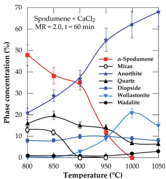
Fig. 10 XRD semi-quantitative analyses of temperature at 60 minutes residence and MR of \text{CaCl}_2 /spodumene of 2.0.
