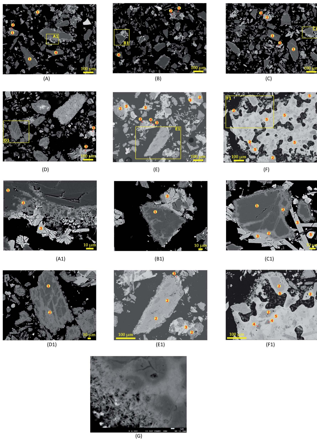
Fig. 8 SEM photomicrographs showing morphological changes of spodumene during 60 min and MR = 1.75 treatment at (A) 750 °C, (B) 800 °C, (C) 850 °C, (D) 950 °C, (E) 1000 °C, (F) 1050 °C and their corresponding spot magnification (A1), (B1), (C1), (D1), (E1) and (F1); (G) fibrous-like structures appearing at the peripheries of spodumene grains during treatment.
