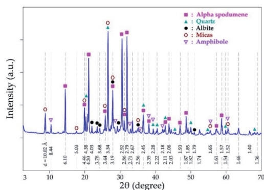
Fig. 3 XRD pattern of spodumene concentrate.
