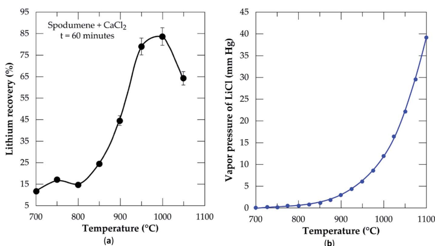
Fig. 6 (a) Percent lithium recovery versus temperature at \text{CaCl}_2/\text{spodumene} molar ratio of 2.0 and 60 min residence time; (b) vapor pressure of lithium chloride versus temperature.
