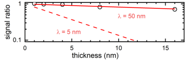
Figure 3: Ratio of the peak signal in Co/Cu(t)/Pt over the peak signal in Co/Pt/Cu(t) as a function of Cu thickness. The ratio is multiplied by the ratio of total absorptions A_{\text{CoPtCu}}/A_{\text{CoCuPt}} . Lines are single exponential decay fits with \lambda = 50 nm (solid) and \lambda = 5 nm (dashed).
