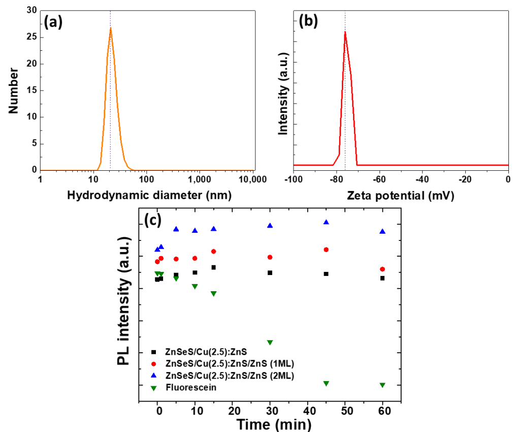
Figure 8. (a) DLS hydrodynamic diameter in number and (b) Zeta potential of ZnSeS/Cu:ZnS/ZnS QDs. (c) Photostability of ZnSeS/Cu(2.5):ZnS, ZnSeS/Cu(2.5):ZnS/ZnS QDs and of fluorescein under the continuous illumination of an Hg–Xe lamp (irradiance of 50 mW/cm 2 ).
