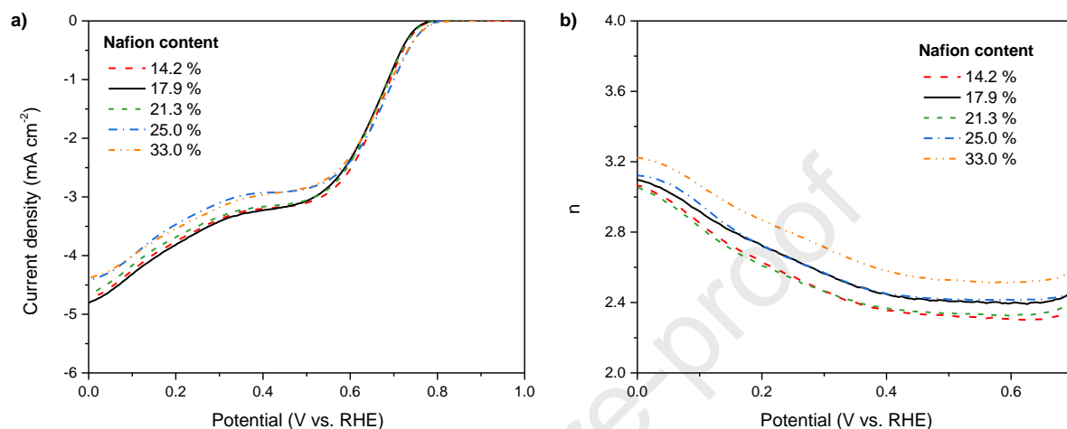
Figure 3. Effect of Nafion® loading (wt.%) on the electrochemical ORR performance of HP-CM: (a) LSV curves and (b) number of electrons transferred ( n ) in 0.1 M KOH solution saturated with \text{O}_2 at 1600 rpm and 5 \text{ mV s}^{-1} . The carbon loading was 0.25 \text{ mg cm}^{-2} .
