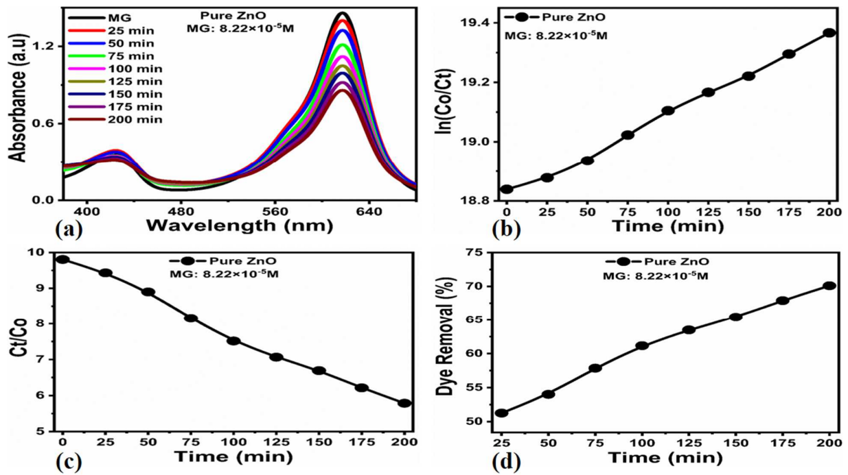
Figure 6. (a) UV-Visible absorption spectra of Pure ZnO (b) 1 st order pseudo-kinetics process of photodegradation of 8.22 \times 10^{-5} \text{ M} MG at different time interval (c) 2 nd order pseudo-kinetics process of photodegradation of MG (d) the dye removal percentage of pure ZnO over MG under sun light source from (25-200 min).
