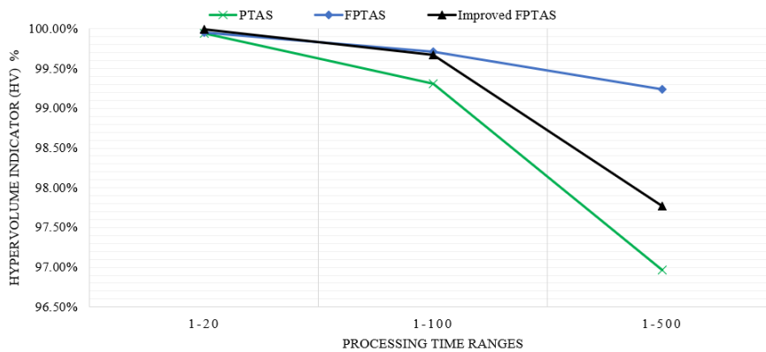
Fig. 12: Quality of our algorithms as a function of processing time with \epsilon=0.2
