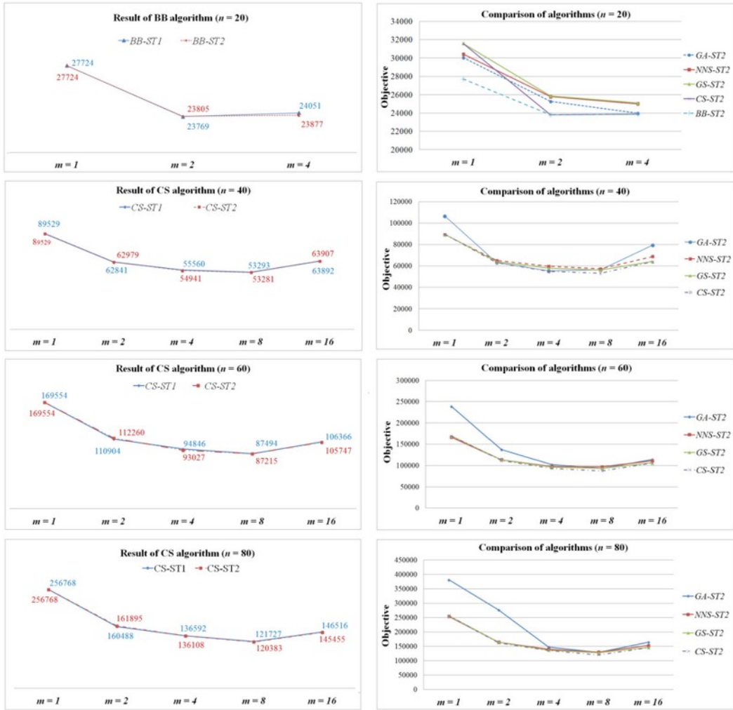
Figure 6. Performances of algorithms for n = 40, 60, 80 (Average results from 8 groups)
