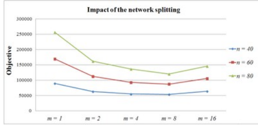
Figure 5. Impact of network decomposition (Average results from 8 groups of 10 instances)
