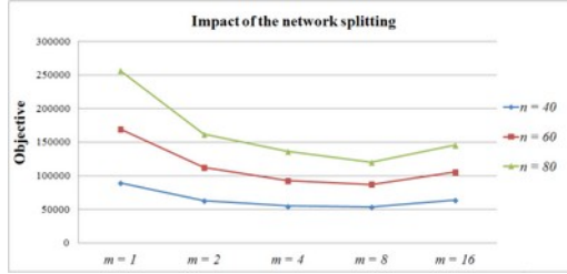
Figure 5. Impact of network decomposition (Average results from 8 groups of 10 instances)
