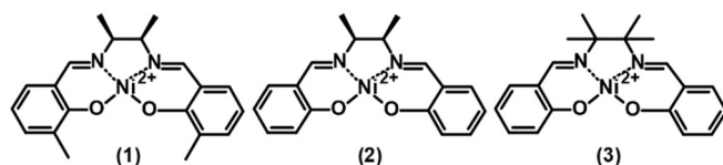
Scheme 1. Structural formulas of (1) meso -NiSaldMe-3dMe, (2) meso -NiSaldMe, and (3) NiSaltMe monomers.
