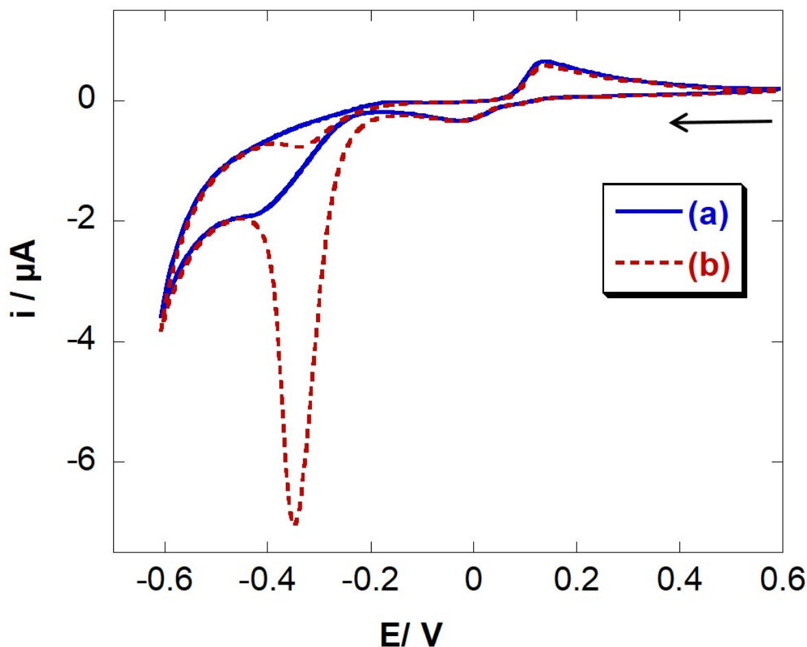
Figure 3. Cyclic voltammograms obtained at bare CPE in 0.1 mol L -1 acetate buffer pH 4.7, scan rate 25mV.s -1
