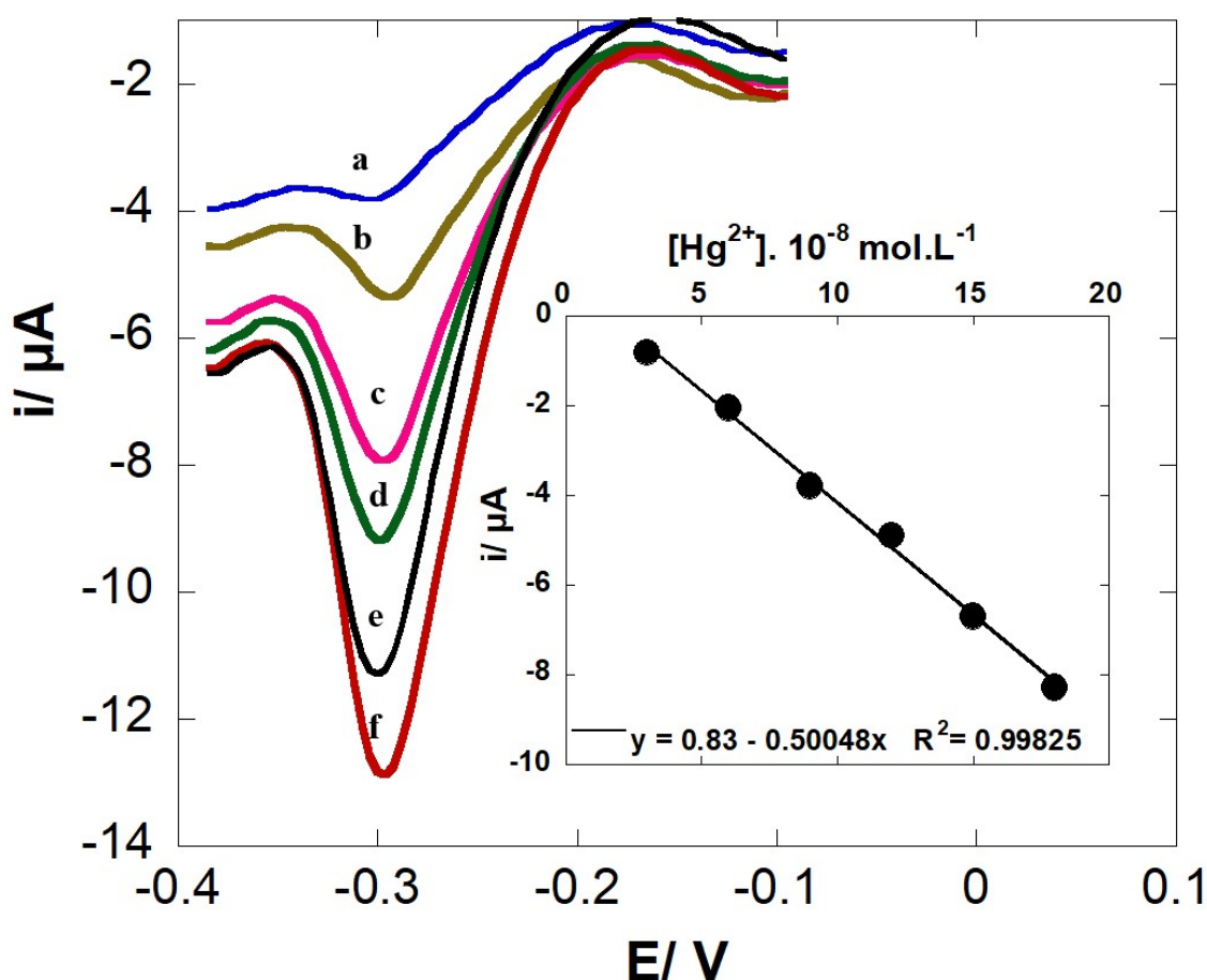
Figure 9. Differential voltammetry curves and calibration curve for different Hg(II) concentrations (a: 3 \times 10^{-8} M, b: 6 \times 10^{-8} mol.L -1 , c: 9 \times 10^{-8} mol.L -1 , d: 1.2 \times 10^{-7} mol.L -1 , e: 1.5 \times 10^{-7} mol.L -1 , f: 1.8 \times 10^{-7} mol.L -1 ), in 0.1 mol.L -1 acetate buffer (pH 4.7), at 0.2% 5-Br-PADAP-CPE
