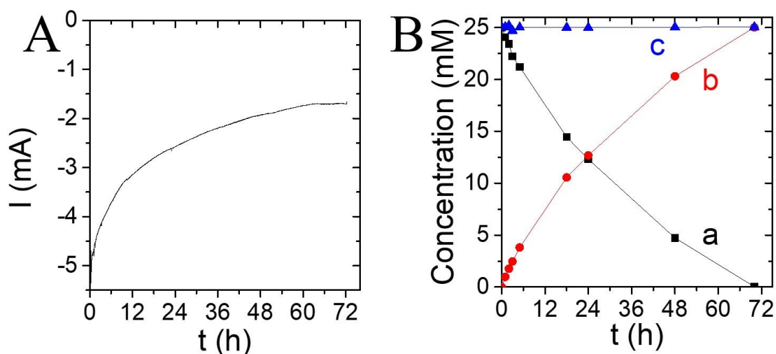
Figure 4. Electroenzymatic synthesis of lactate from 25 mM pyruvate in 100 mL solution containing 10 \mu\text{M} \text{NAD}^+ (and 50 mM PBS, pH 7.2) in the hybrid flow cell provided with two CP-MWCNT-bpy-Rh electrodes and one enzymatic CP-MWCNT-LDH (500 units) layer (Experiment 3). (A) Variations of the current in the run. (B) Time variations of the concentrations of (a) pyruvate, (b) lactate, and (c) the sum pyruvate and lactate, as determined by HPLC.
