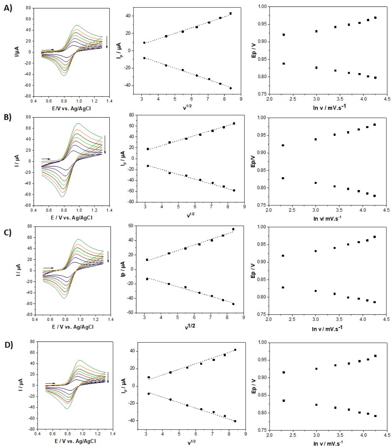
Figure 5. Cyclic voltammograms of [\text{Fe}(\text{bpy})_3]^{2+}\text{SO}_3^-@ \text{SiO}_2 functionalized films recorded at potential scan rates of 10, 20, 30, 40, 50, 60 and 70 \text{mV s}^{-1} in an aqueous electrolyte solution containing 0.1 M \text{NaNO}_3 . Left: CVs of the films prepared from various MPTMS/TEOS ratios (total concentration of silane precursors: 200 mM): 30/70 (A); 20/80 (B); 10/90 (C); 5/95 (D). Middle: Dependence of the peak current with the square root of the potential scan rate. Right: Evolution of peak potentials as a function of the logarithm of potential scan rate.
