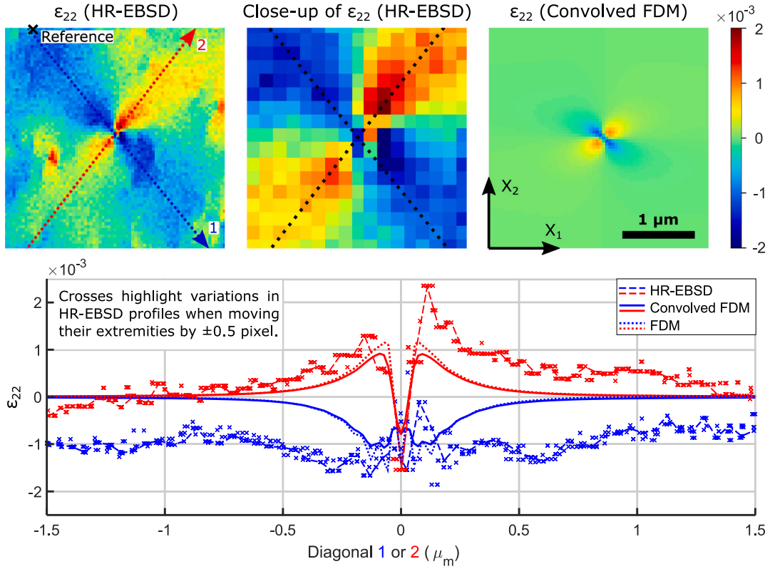
Fig. 8. Elastic strain \epsilon_{22} of the threading screw dislocation measured by HR-EBSD and predicted by the field dislocation mechanics model.
