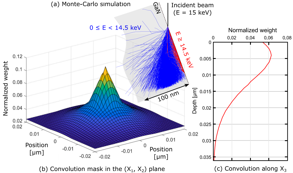
Fig. 3. (a) Monte-Carlo simulation of the backscattered electron (BE) trajectories performed with the CASINO software [25]. (b) Convolution mask in the (X_1, X_2) plane. (c) Convolution mask in depth.
