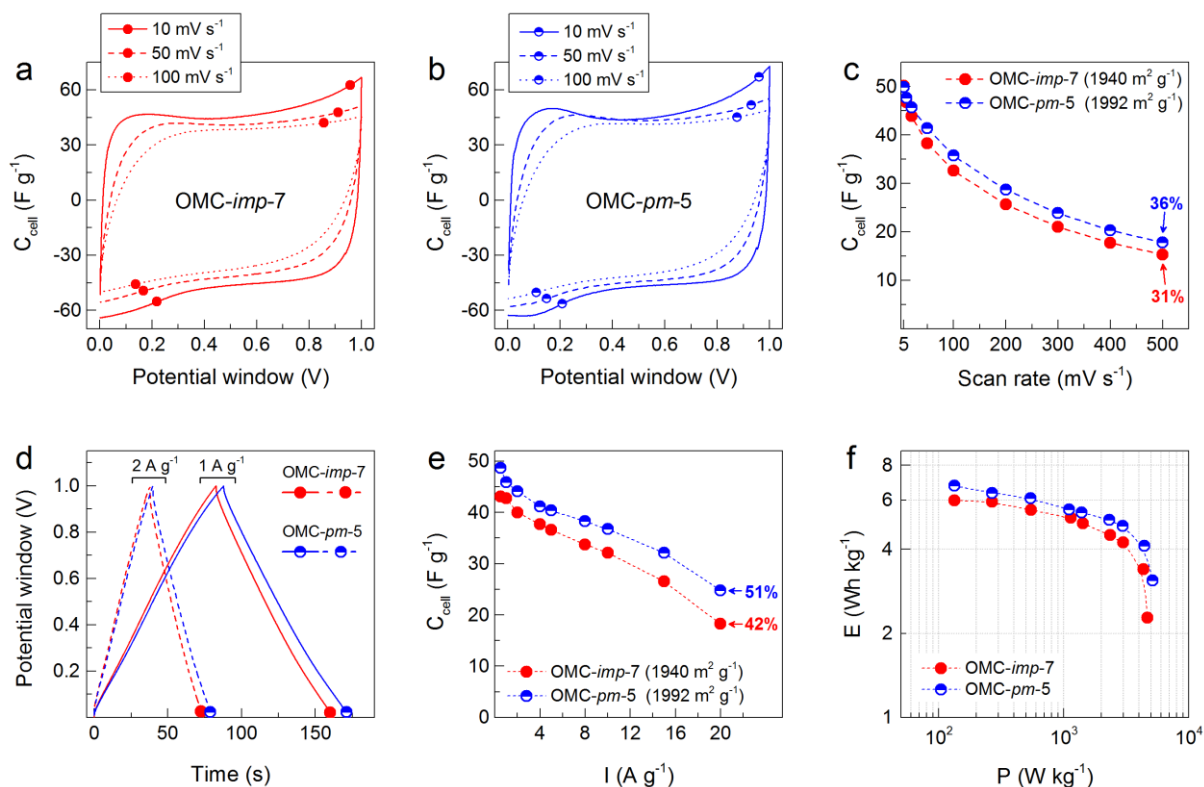
Figure 7. Electrochemical performance of KOH-activated OMCs by the impregnation and physical mixing incorporation routes, OMC- imp-7 and OMC- pm-5 , respectively. CV curves at different scan rates for (a) OMC- imp-7 and (b) OMC- pm-5 ; (c) specific cell capacitance ( C_{cell} ) as a function of scan rate; (d) charge-discharge curves at 1 and 2 A g^{-1} ; (e) C_{cell} as a function of specific applied current ( I ); the capacitance retention at 500 mV s^{-1} for CV curves and 20 A g^{-1} for GCD, and S_{NLDFT} values for each material are also indicated; (f) Ragone-like plot.
