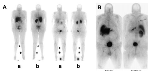
Figure 15: (A) Planar scintigrams of patients at 4 hours p.i. of ^{111}\text{In} In-4 (183 MBq) (a : anterior, b: posterior). Image reprinted with permission from [141]. Copyright 2022 SNMMI. (B) SPECT images of 57-year-old man with pulmonary metastases from renal cell carcinoma at 1-2 hours p.i. of ^{99m}\text{Tc} Tc-23 (555 MBq). Image reprinted with permission from [142]. Copyright 2022 SNMMI
