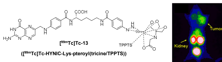
Figure 9: Chemical structure of [^{99m}\text{Tc}]\text{Tc-13} and SPECT image of KB tumor-bearing mice at 2 hours p.i. of [^{99m}\text{Tc}]\text{Tc-13} (7.4 MBq). Image reprinted with permission from [130]. Copyright 2022 Elsevier
