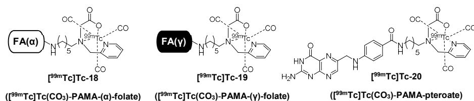
Figure 12: Chemical structures of [ 99m Tc]Tc-18, [ 99m Tc]Tc-19 and [ 99m Tc]Tc-20 [102,135]
