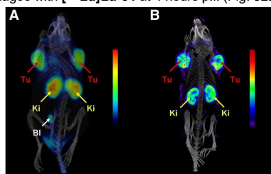
Figure 32: (A) PET/CT images of KB tumor-bearing mice at 4 hours p.i. of ^{44}\text{Sc} Sc-54 (25 MBq) and (B) SPECT/CT images of KB tumor-bearing mice at 4 hours p.i. of ^{177}\text{Lu} Lu-54 (35 MBq). Images reprinted with permission from [183]. Copyright 2022 SNMMI
