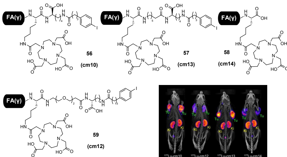
Figure 3411: Chemical structures of 56 , 57 , 58 and 59 and SPECT/CT images of KB tumor-bearing mice at 24 hours p.i. of [ ^{177}\text{Lu} ]Lu- 56 , [ ^{177}\text{Lu} ]Lu- 57 , [ ^{177}\text{Lu} ]Lu- 58 and [ ^{177}\text{Lu} ]Lu- 59 (50 MBq). Reprinted with permission from Siwowska et al. Mol. Pharm. 14 (2017) 523–532. Copyright 2022 American Chemical Society.
