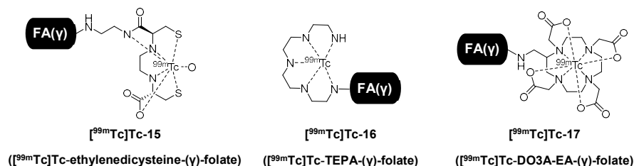
Figure 11: Chemical structures of [ 99m Tc]Tc-15, [ 99m Tc]Tc-16 and [ 99m Tc]Tc-17 [132–134]
