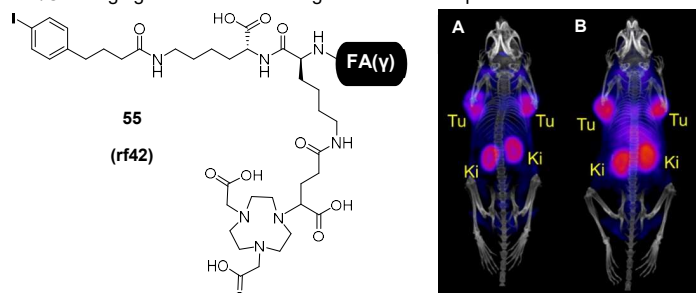
Figure 31: Chemical structure of 55 and PET/CT images of KB tumor-bearing mice at 2 hours p.i. of ^{64}\text{Cu} Co-55 (3.5-7 MBq) (A) and ^{68}\text{Ga} Ga-55 (5 MBq) (B). Reprinted with permission from Farkas et al. Mol. Pharm. 13 (2016) 1979–1987. Copyright 2022 American Chemical Society
