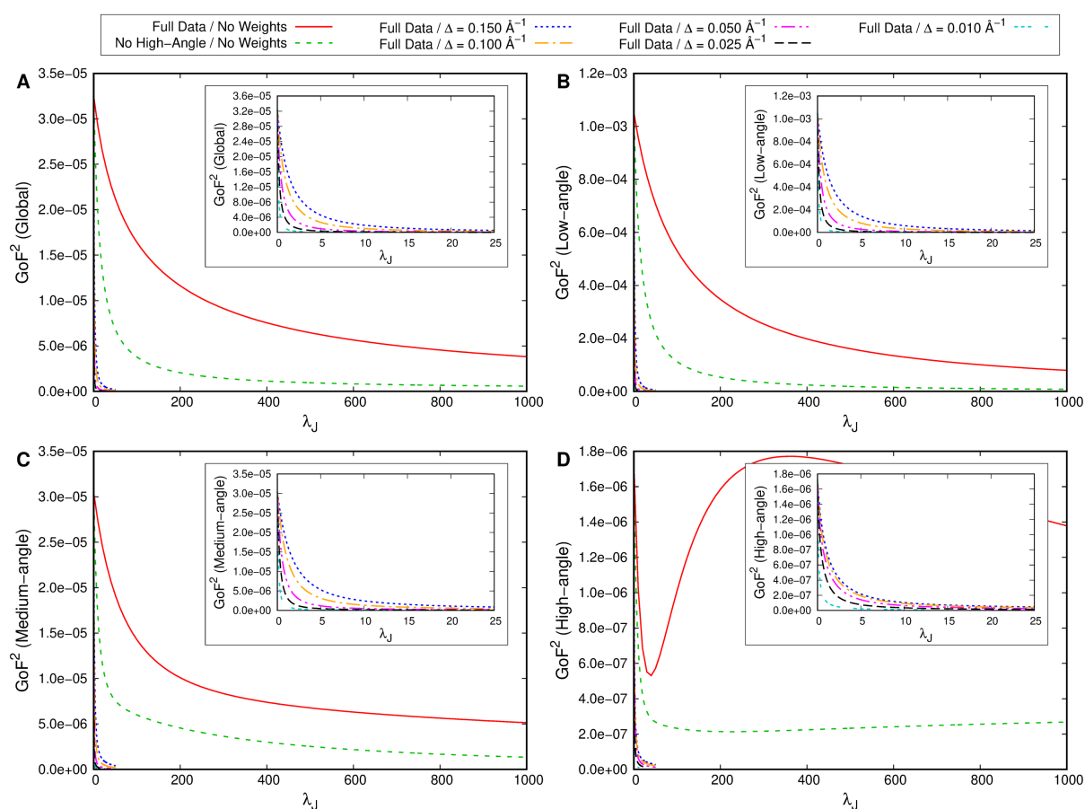
Figure 3 \text{GoF}^2 as a function of \lambda_j in different resolution ranges for the XRW calculations performed with structure factor amplitudes corresponding to the gas-phase CCSD/UGBS electron density of HCN: (A) global \text{GoF}^2 , (B) low-angle \text{GoF}^2 , (C) medium-angle \text{GoF}^2 , and (D) high-angle \text{GoF}^2 . The insets show the zoomed plots only for the XRW calculations carried out with the weighting scheme.
