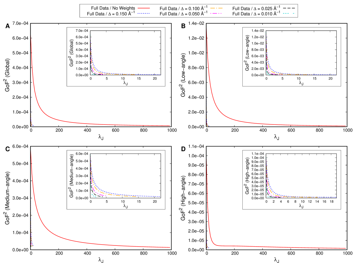
Figure 6 \text{GoF}^2 as a function of \lambda_J in different resolution ranges for the XRW calculations performed with structure factor amplitudes corresponding to the periodic B3LYP/cc-pVTZ electron density of urea ( (\sin\theta/\lambda)_{\max} = 2.00 \text{ \AA}^{-1} ): (A) global \text{GoF}^2 , (B) low-angle \text{GoF}^2 , (C) medium-angle \text{GoF}^2 , and (D) high-angle \text{GoF}^2 . The insets show the zoomed plots only for the XRW calculations carried out with the weighting scheme.
