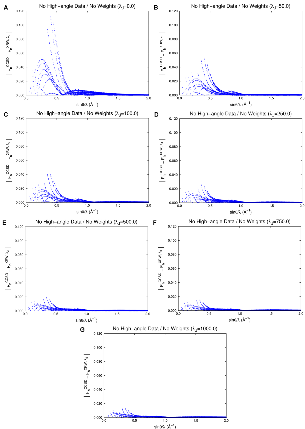
Figure S2 Absolute differences between calculated and reference structure factor amplitudes at different values of \lambda_j for the XRW calculation performed without applying the proposed weighting scheme and by exploiting only the low- and medium-angle sets of X-ray diffraction data corresponding to the gas-phase CCSD/UGBS electron density of HCN.
