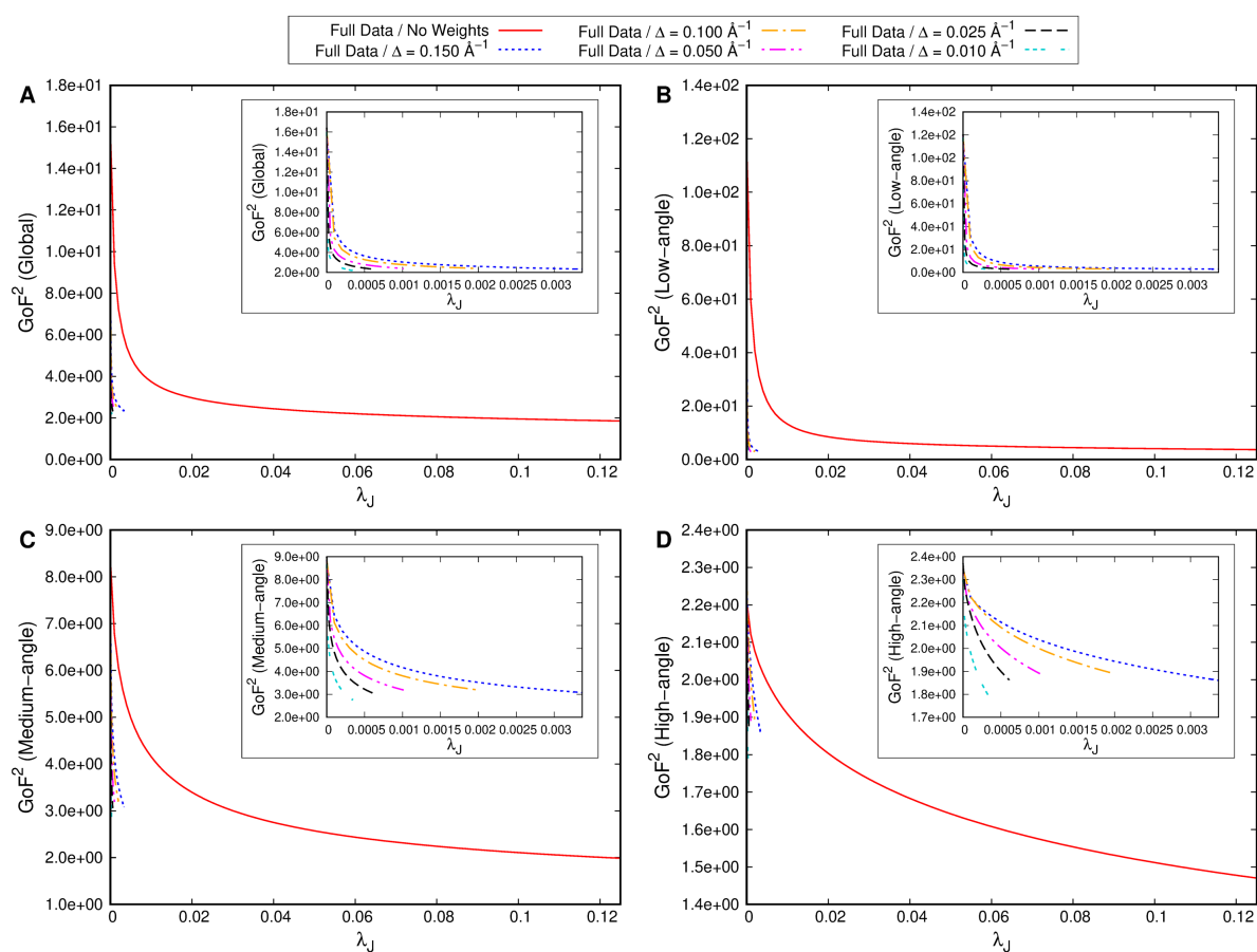
Figure 4 GoF 2 as a function of \lambda_j in different resolution ranges for the XRW calculations performed with experimental structure factor amplitudes for urea: (A) global GoF 2 , (B) low-angle GoF 2 , (C) medium-angle GoF 2 , and (D) high-angle GoF 2 . The insets show the zoomed plots only for the XRW calculations carried out with the weighting scheme.
