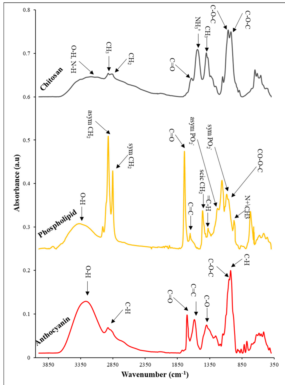
Figure 5. FTIR spectrum of anthocyanin, phospholipid, and chitosan.
