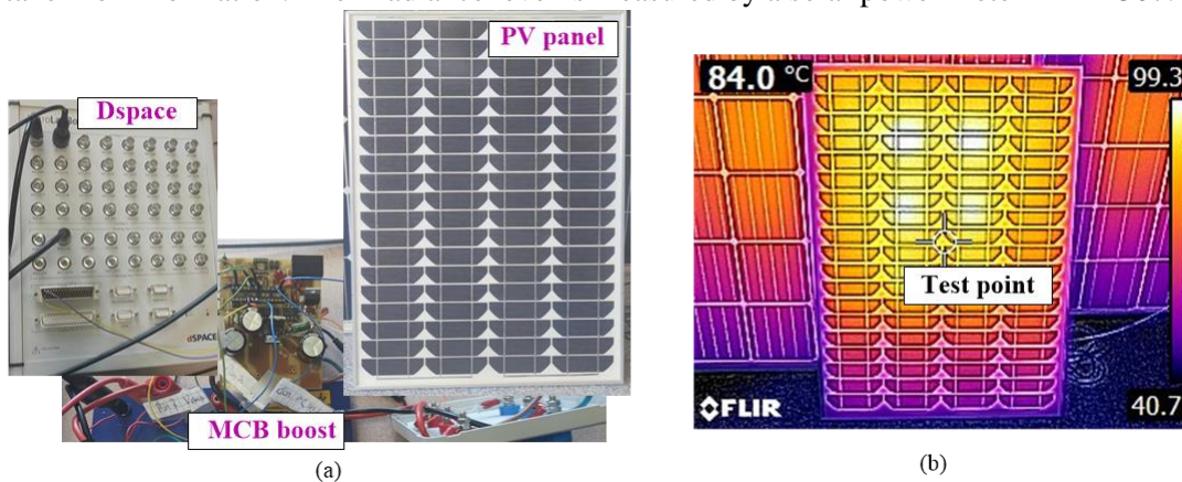
Fig. 5 (a) Experimental platform (b) Operating temperature based on FLIS E8
