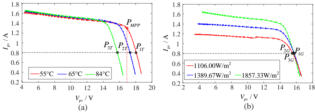
Fig. 6 Experimental injecting points (a) inject current-perturbation signal; (b) inject voltage-perturbation signal
