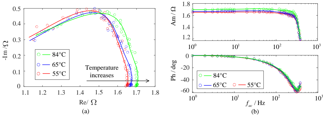
Fig. 7 Experimental results of different operating temperatures (a) Nyquist curves; (b) Bode diagrams
