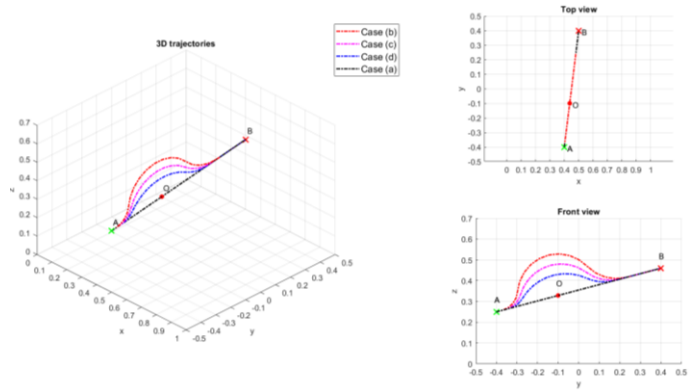
Figure 5.1 UR10e trail trajectories: (a) linear trajectory; (b), (c) and (d) obstacle avoidance trajectories; Figure 5.2 Resulting end-effector positions in the Cartesian space
