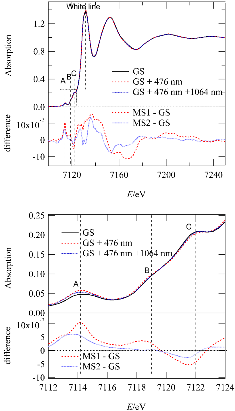
Figure 1: XAS spectra for an 80 \mu\text{m} thick crystal (a-cut, polarization of X-ray beam perpendicular to the c -axis of the crystal, i.e. with a component parallel to the Fe–N–O direction): GS (black line), after irradiation with 476 nm light (red dashed line) and subsequent irradiation with 1064 nm (blue dotted line). A, B, C denote pre-edge features at 7114, 7119, and 7122 eV, respectively. (Top) Full range 7100 – 7250 eV and corresponding difference spectra. (Bottom) Zoom in the range 7110 – 7124 eV.
